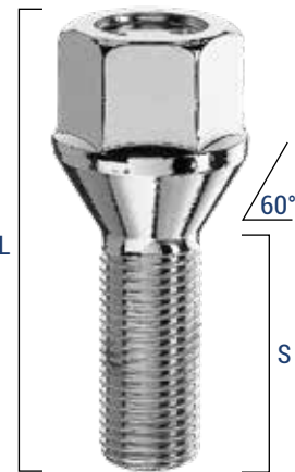
CONE SEAT 60° 19 mm (3/4") HEX - M12X1,25
